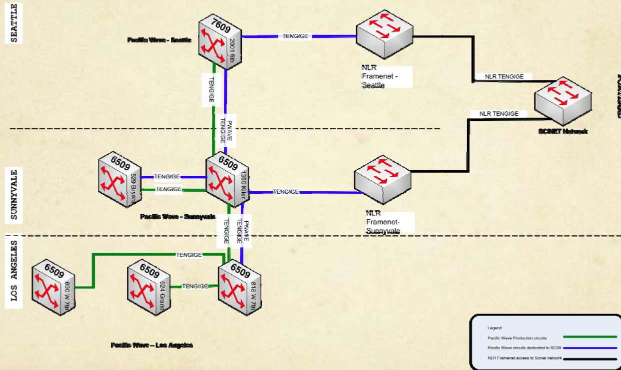
Pacific Wave access to SC09 via NLR Framenet
