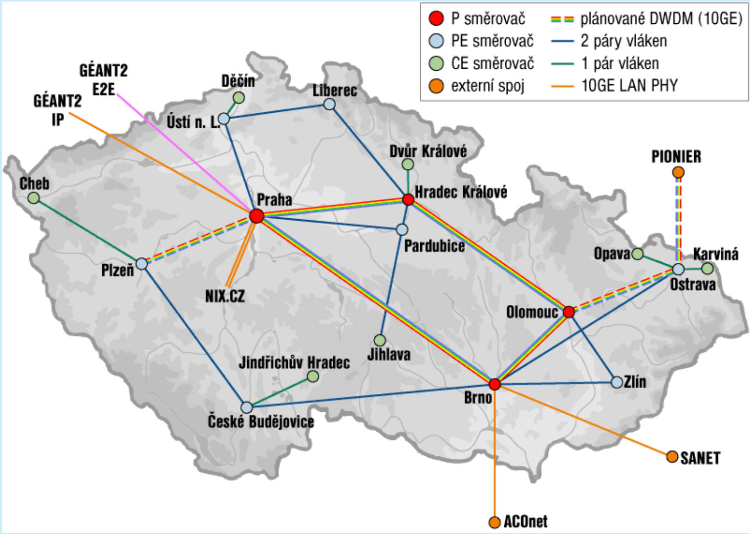
CESNET2 Planed DWDM Development in 2006
